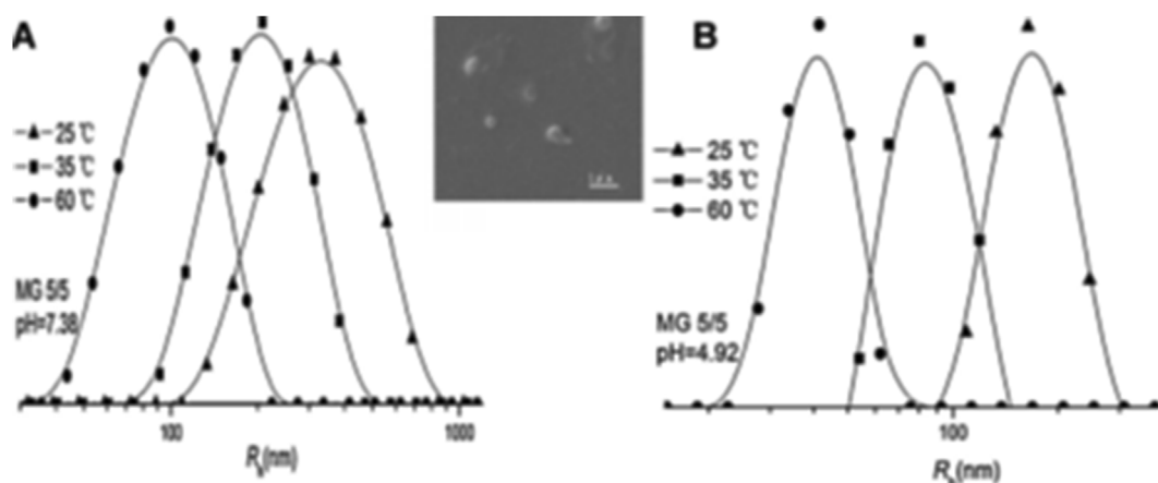
Fig. 3. Hydrodynamic radius distributions for MG5/5 in aqueous solution of pH 7.38 and pH 4.92 at 25, 35 and 60 °C, respectively. Scanning electron microscopy (SEM) image of MG5/5 is in the inset. Reproduced with permission from Ref. [41].
